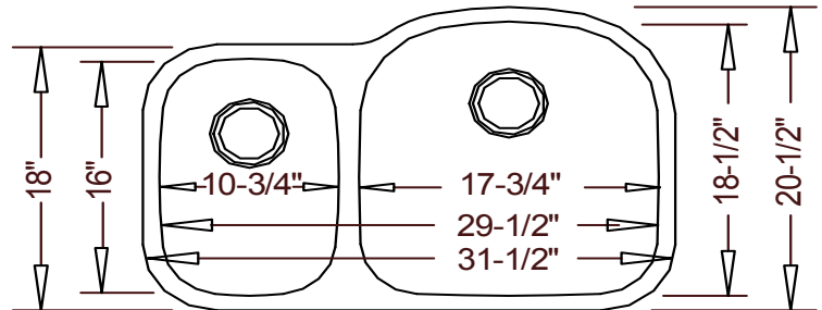
Product Diagram
