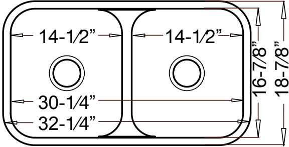
Product Diagram
