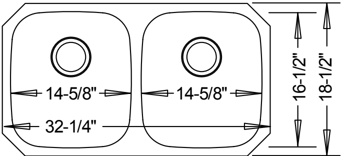
Product Diagram
