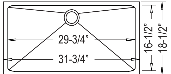
Product Diagram
