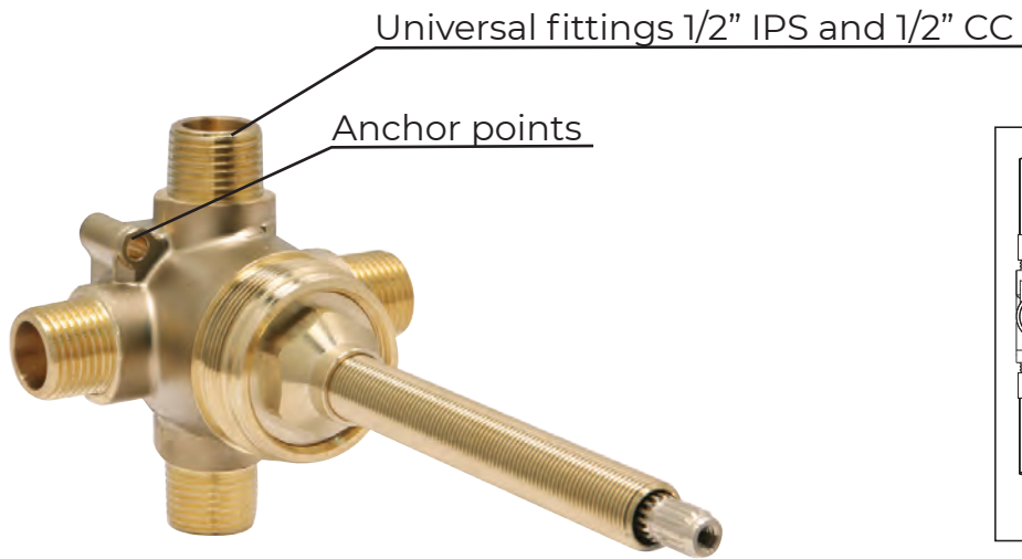
P2423199 Four Port Diverter Valve
